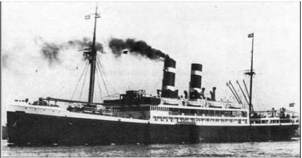
The "Simon Bolivar" (KNSM - 1927 / 1939. Built by Rotterdamsche Droogdok Mij., Rotterdam 8309 grt; 134x18m; 14.5kn; 238 passengers in 3 classes). Employed in Hamburg-Central America service (Colón Line) alternating with cruises.
